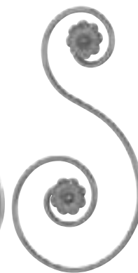
H.420 X L.220 mm. Art. 01.131.29 Ø 10 Art. 01.131.67 Ø 12 Art. 01.131.68 Ø 14
